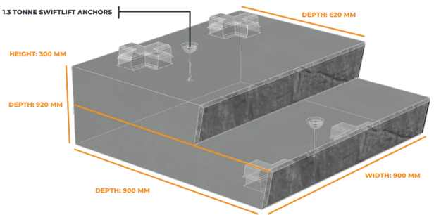
4SBC900STRCAP STAIR STONEBLOC CROATIA CAPPER BLOCK 300 X 150, 105KG
