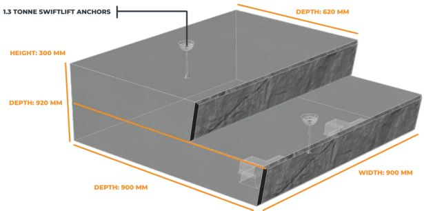
4SBC900STRFT STAIR STONEBLOC CROATIA FLAT TOP BLOCK 900 X 300, 518KG
