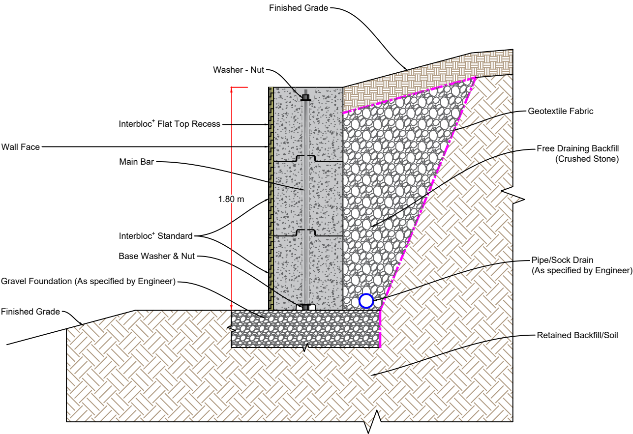
INTERBLOC + ® Retaining Wall Cross Section Vertical Reinforcing - Top & Bottom Kits
