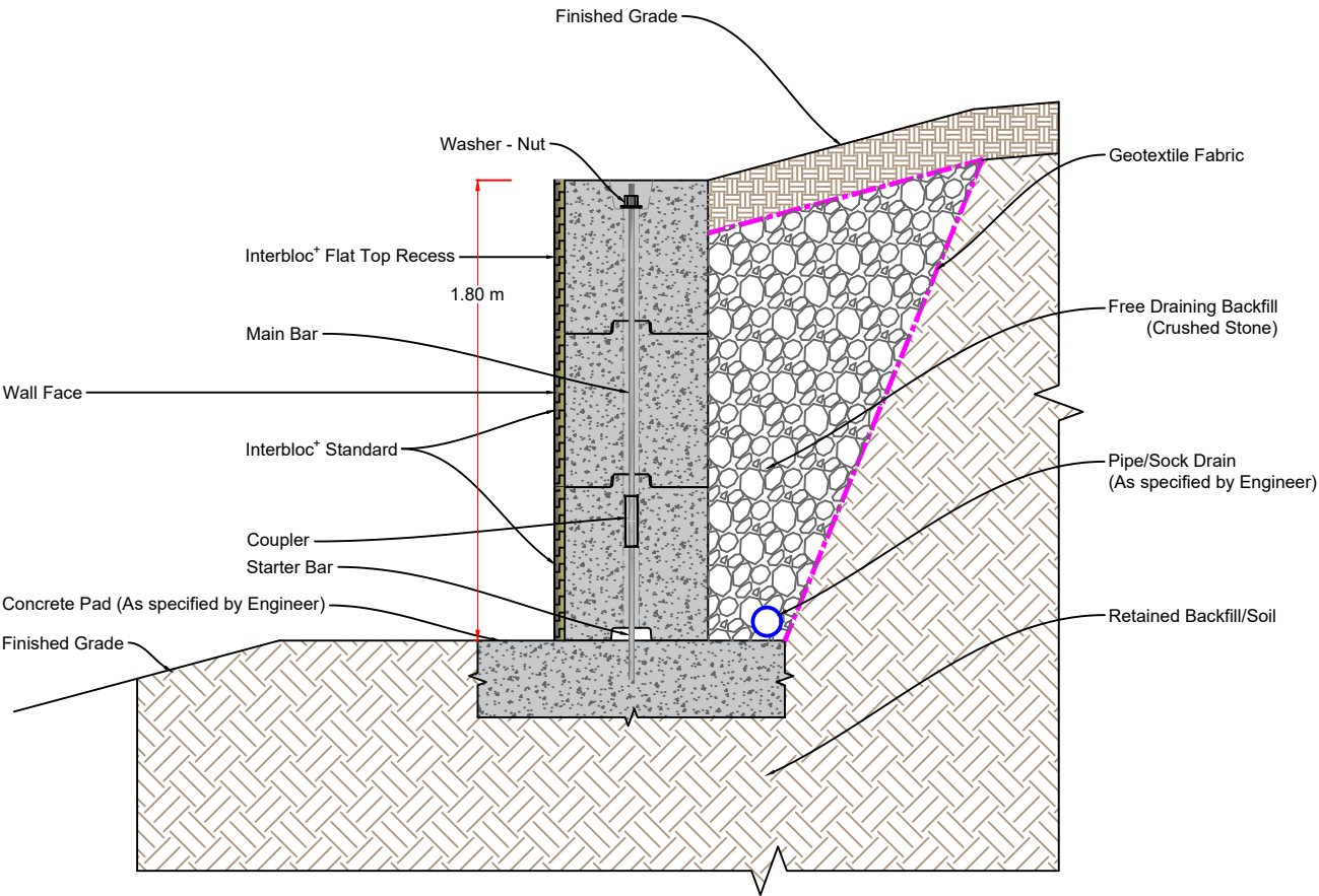
INTERBLOC + ® Retaining Wall Cross Section Vertical Reinforcing - Standard Kits
